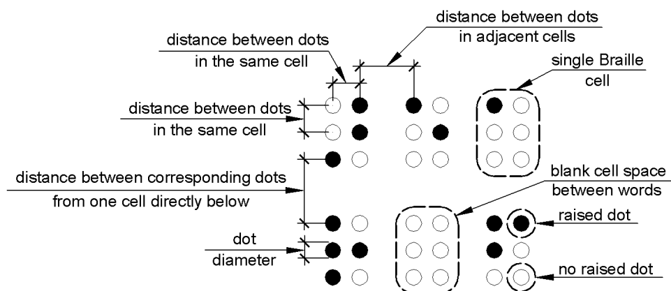
Figure 703.3.1 Braille Measurement
