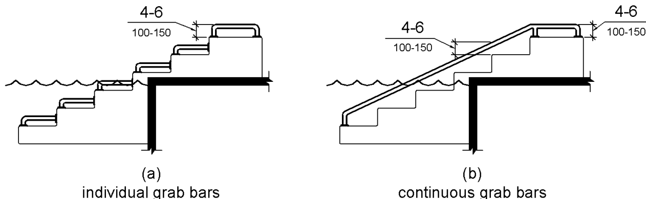
Figure 1009.5.7 Grab Bars
