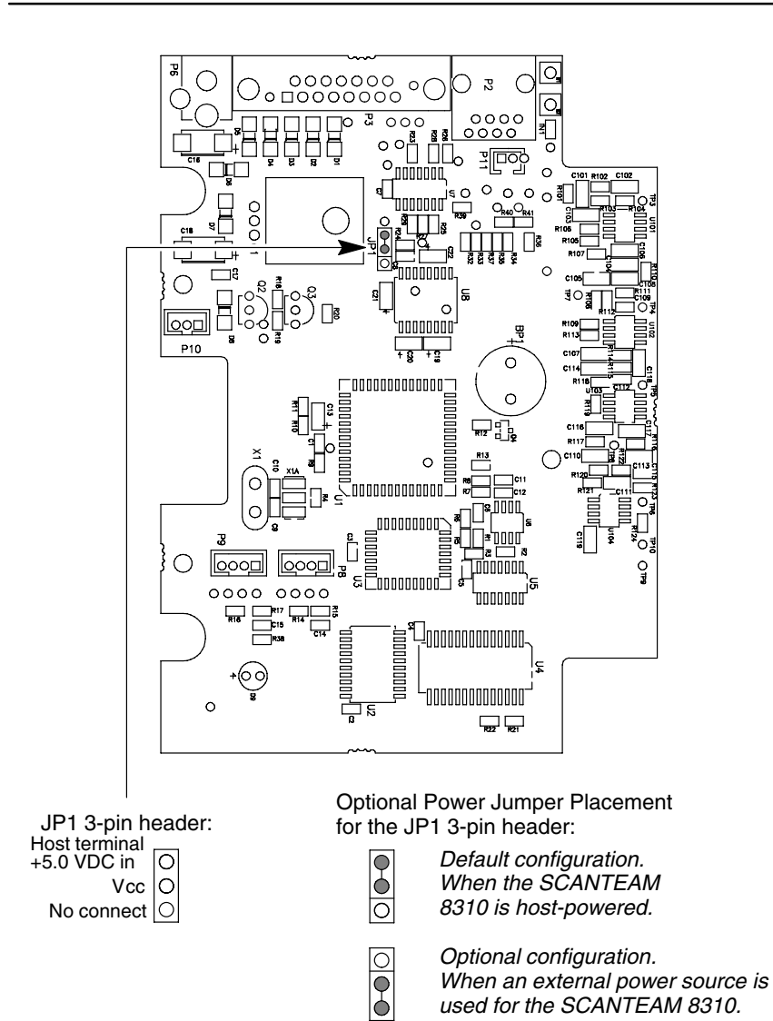
Figure 14 SCANTEAM 8310 PC Board
