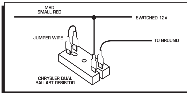
Figure 8 Wiring the Dual Ballast Resistor for Run-On.
