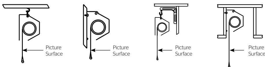
Ceiling Mounted
