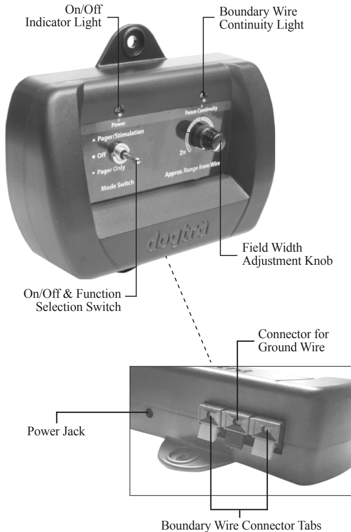
E-FENCE 3500 Transmitter
