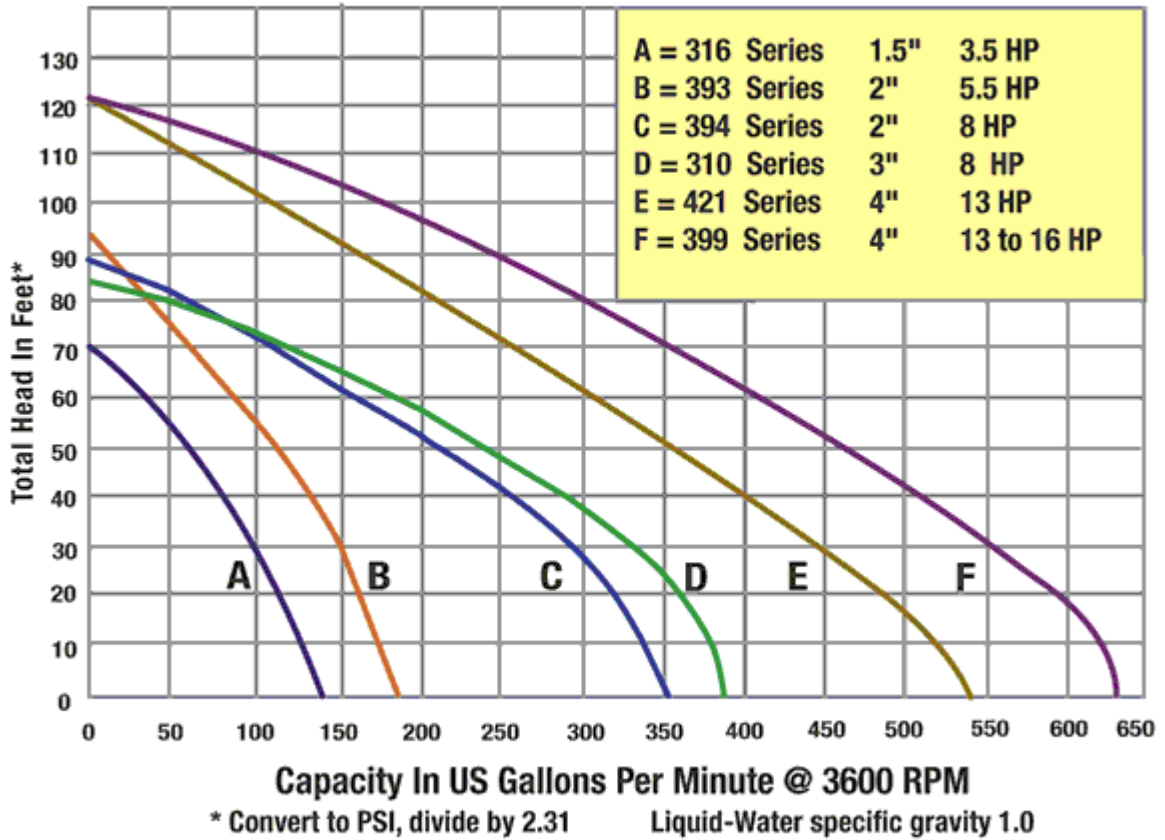
Performance of Engine Driven Trash Pumps
