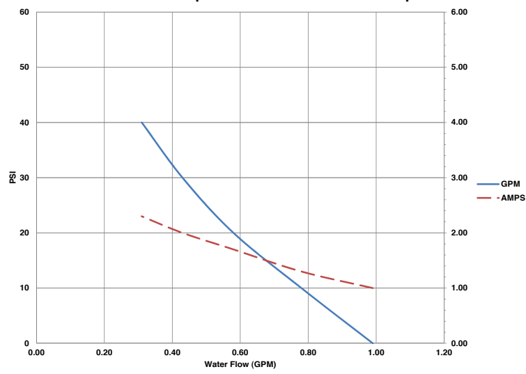
BevJet Compact - Head Flow Curve & Amps
