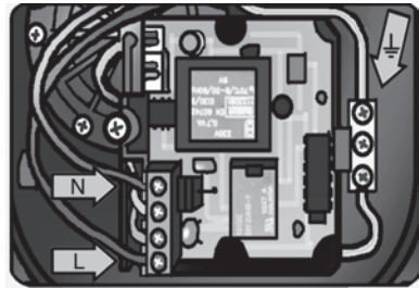
Fig. 10 Electrical connection
