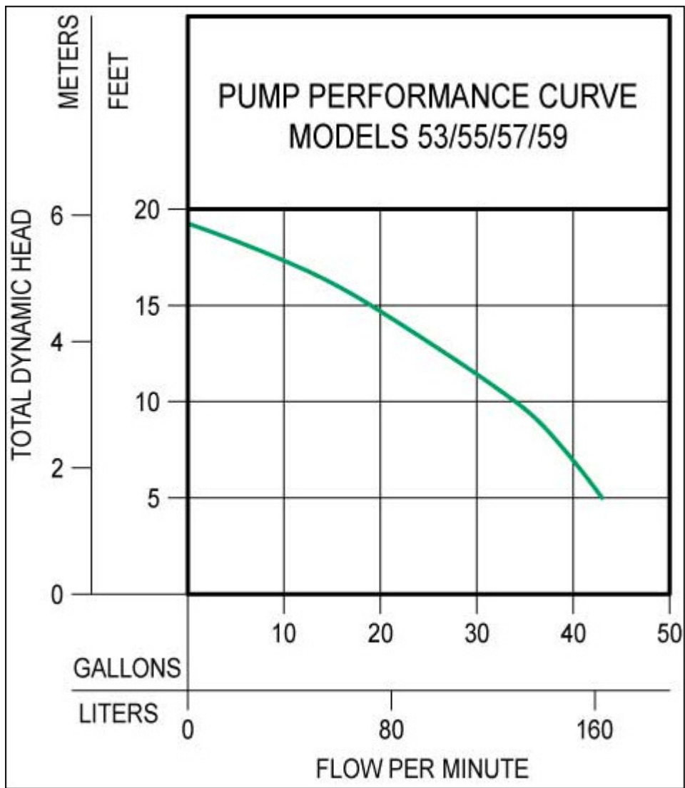
Pump Performance Curve Models 53, 55, 57, 59
