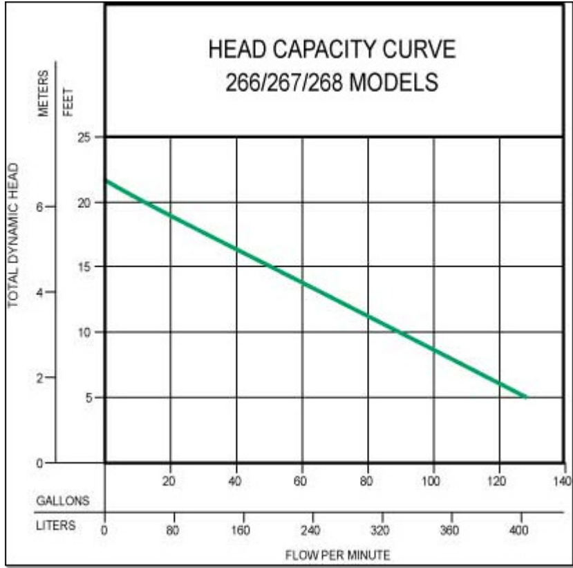
Pump Performance Curve Models 266, 267, 268
