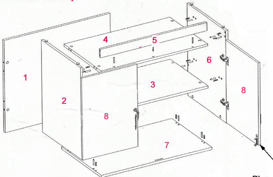
Plunger Lock
