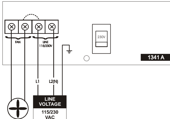
Figure 1: Wiring Diagram
