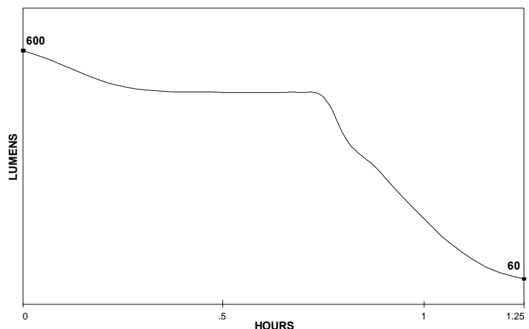
Scorpion HL PERFORMANCE CURVE
