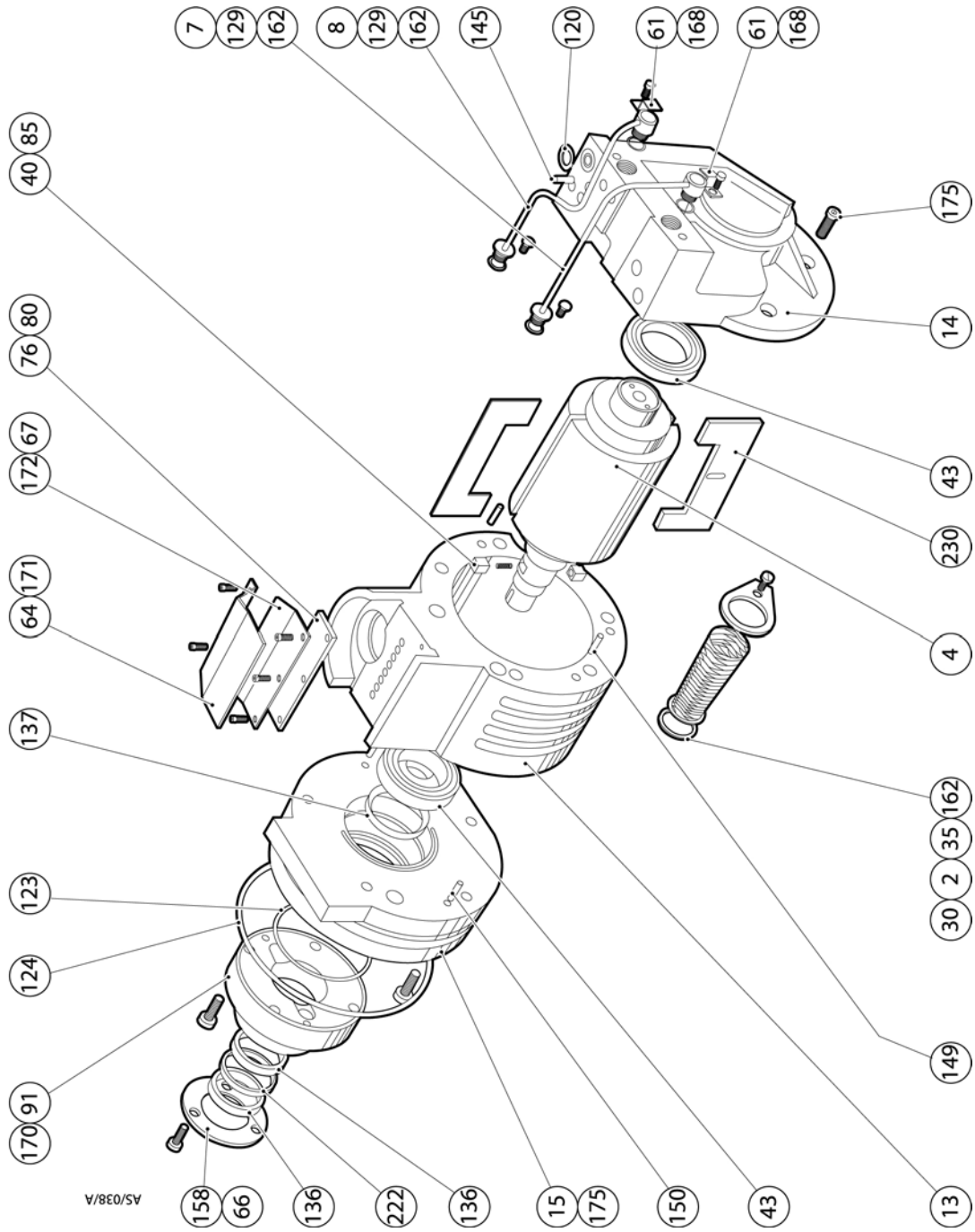
Figure 6 - (E) E1M40 HV stator sub-assembly
