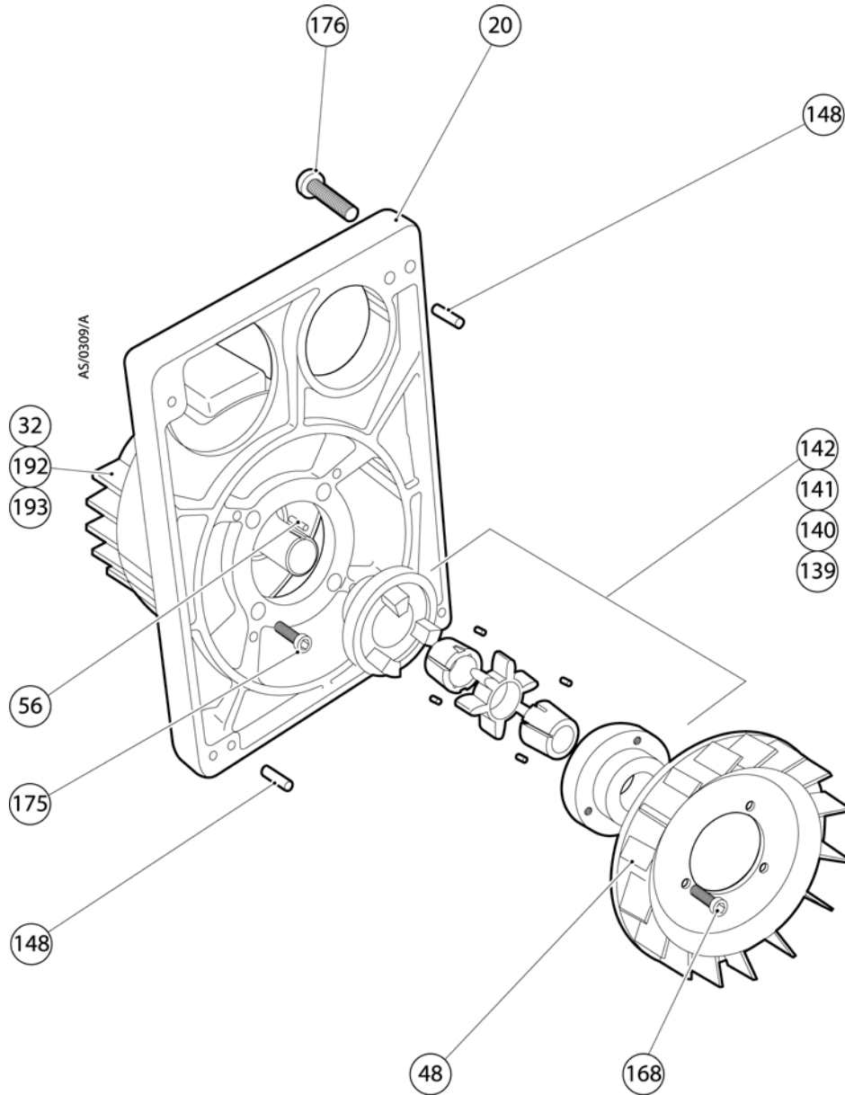
Figure 7 - (G) E1M40 motor plate sub-assembly
