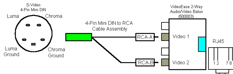
Pin Configuration - S-Video to RJ45
