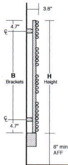
Side View Piping Dimensions
