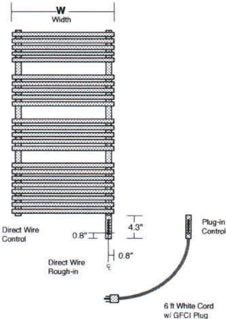
Front View Piping Dimensions
