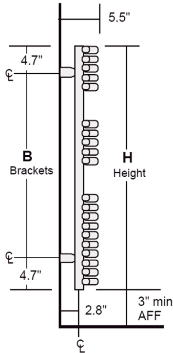
Side View Dimensions
