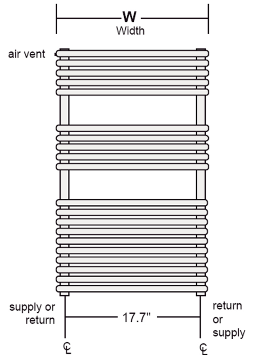
Front View Dimensions
