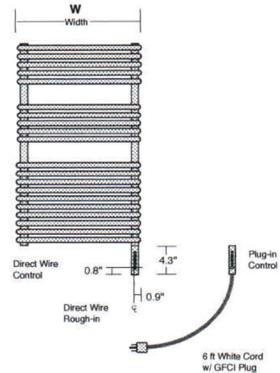
Front View Piping Dimensions
