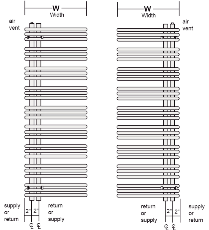
Front View Lefthand & Righthand Dimensions
