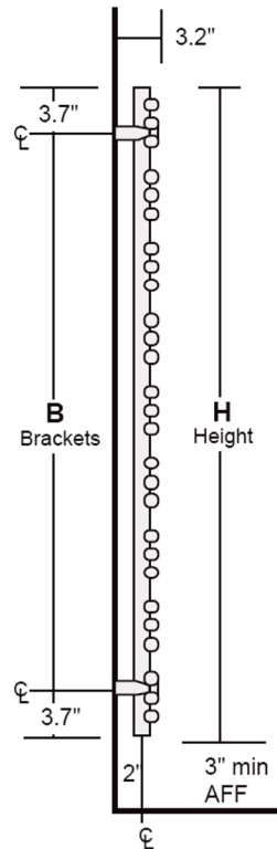
Side View Dimensions
