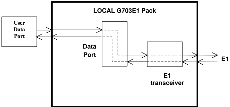
Figure 1-4: Transparent Timing
