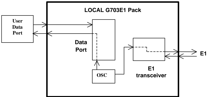
Figure 1-2: Internal Timing
