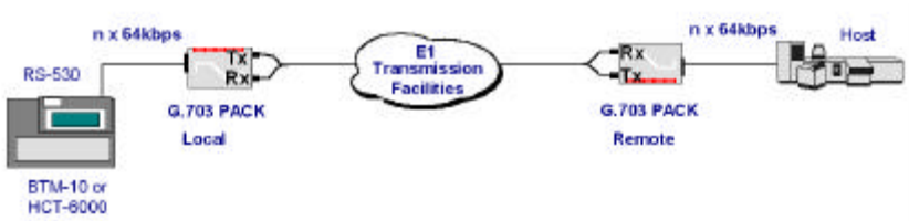
Figure 3-2: Link testing with BTM-10 or HCT-6000
