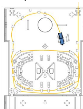
Figure 13: Fiber cable installation (with LAN cable protection holder)
