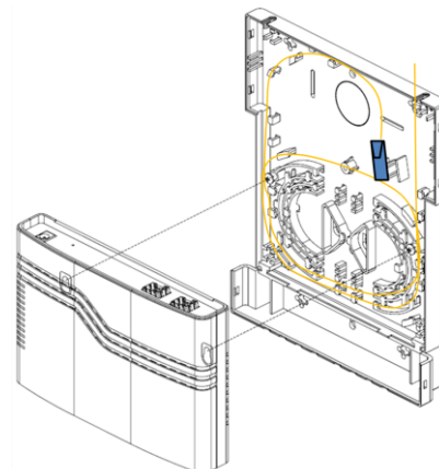
Figure 16: Install the device onto the cable tray (with LAN Cable Protection Holder)
