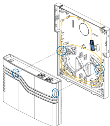
Figure 15: Install the device onto the cable tray
