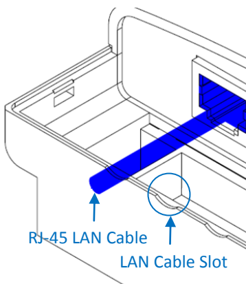
Figure 19: Install LAN cable
