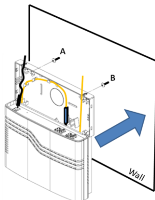
Figure 26: Mount the device on the wall
