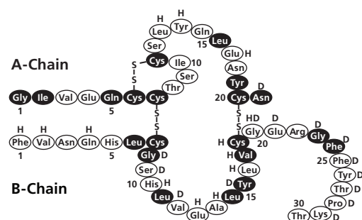
Figure 1: Structural formula of NOVOLIN® R
