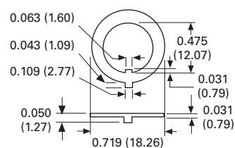
Locking Ring
