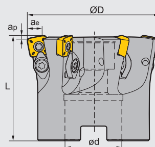
S-type insert, arbor mounting
