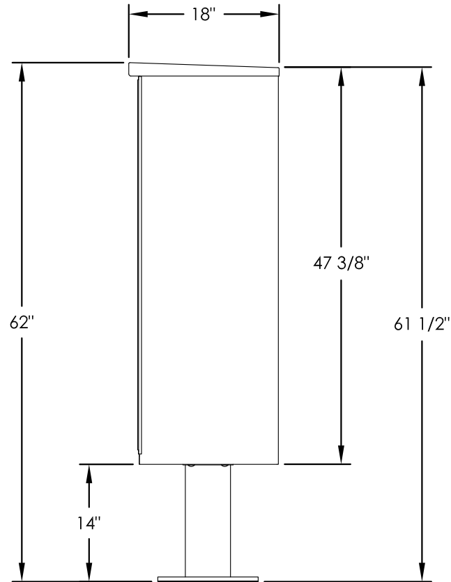
SIDE VIEW
