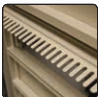
Aluminum comb prevents mail fishing from the outgoing mail collection compartment.
