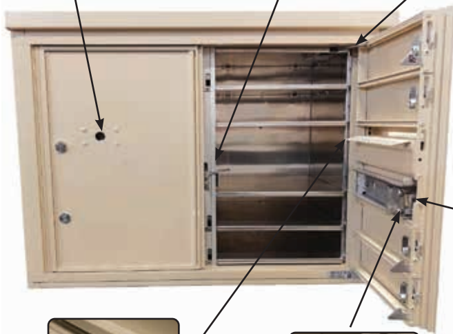
Fully integrated parcel locker(s) with key trapping lock
