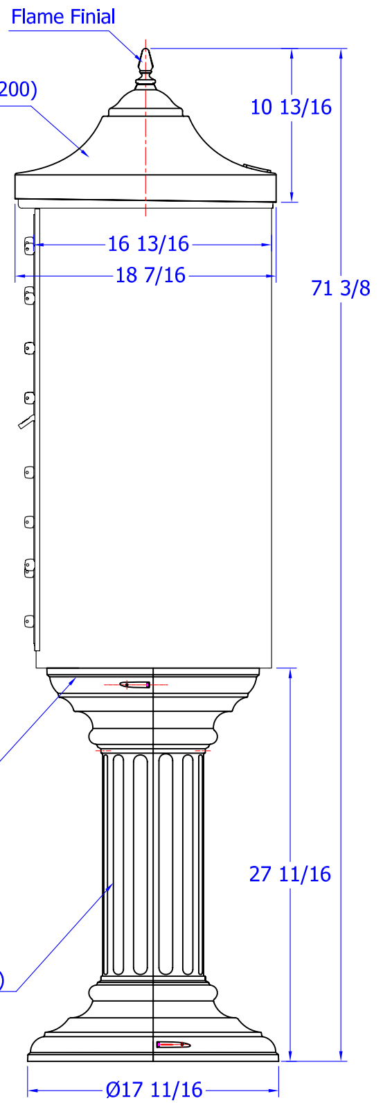
Side View
