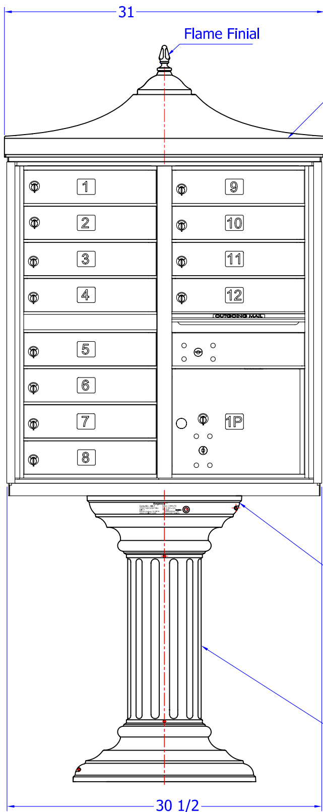
Front View
