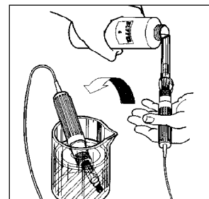
FIGURE 21 Adding pH buffer solution to sensor in a clean container for calibration.
