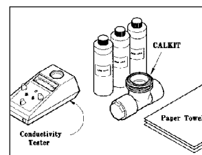
FIGURE 9 CALKIT shown with tester and paper towels.
