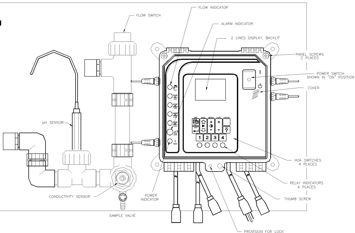
FIGURE 8 Front Panel
