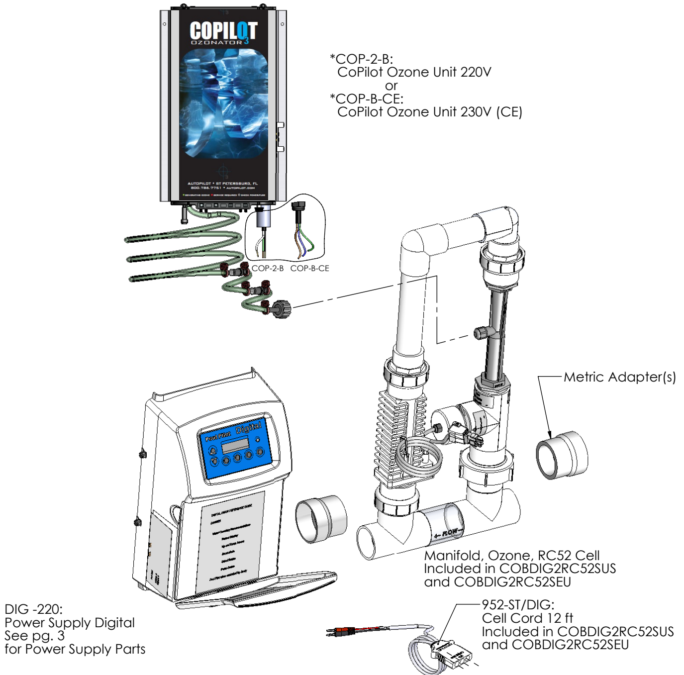
CoPilot with DIG-220 Systems
